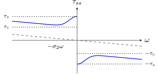
Figure 6: Steady-state friction \tau_{ss}(\omega) = -g(\omega) \operatorname{sgn}(\omega) - \sigma_2 \omega . Stiction torque \tau_s at \omega=0 drops to Coulomb level \tau_c over velocity scale \omega_s (Stribeck effect). Friction opposes motion.
